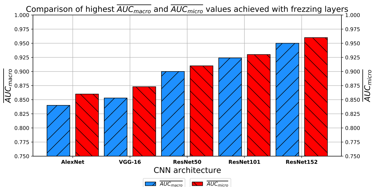
Figure 29. Comparison of highest \overline{AUC}_{macro} and \overline{AUC}_{micro} achieved with every CNN architecture and freezing layers.
