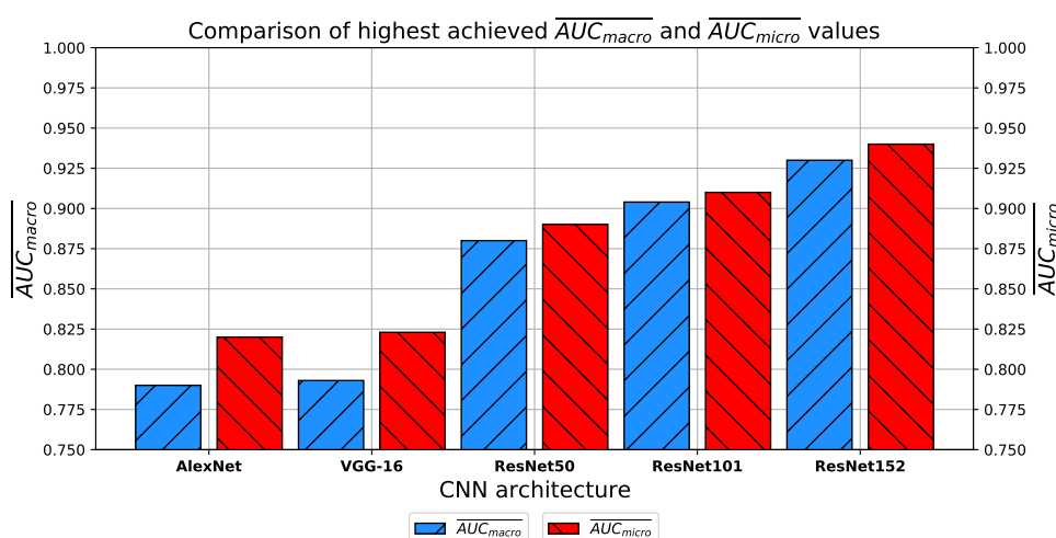
Figure 28. Comparison of highest \overline{AUC}_{macro} and \overline{AUC}_{micro} achieved with every CNN architecture.
