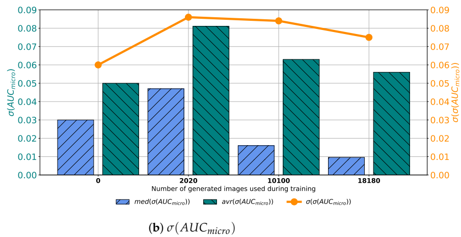
Figure 11. Median, average AUC_{micro} and standard deviation of AUC_{micro} and \sigma(AUC_{micro}) for the case of VGG-16 trained with images generated by GAN in 100 epochs.
